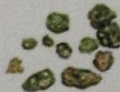
Peridot
